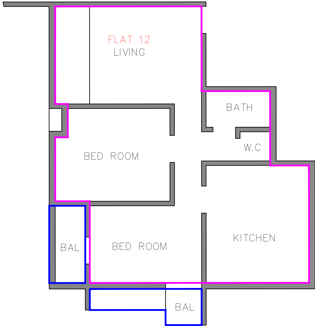
FLAT 12 RERA CARPET
